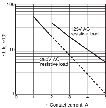
2. Life curve
